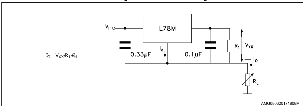
Figure 18: Constant current regulator
