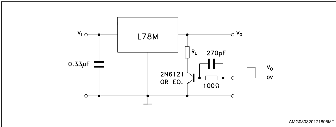
Figure 7: Ripple rejection
