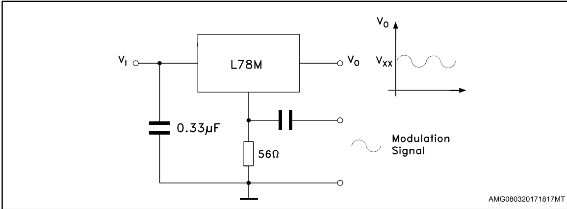
Figure 27: Power AM modulator (unity voltage gain, IO ≤ 0.5)
