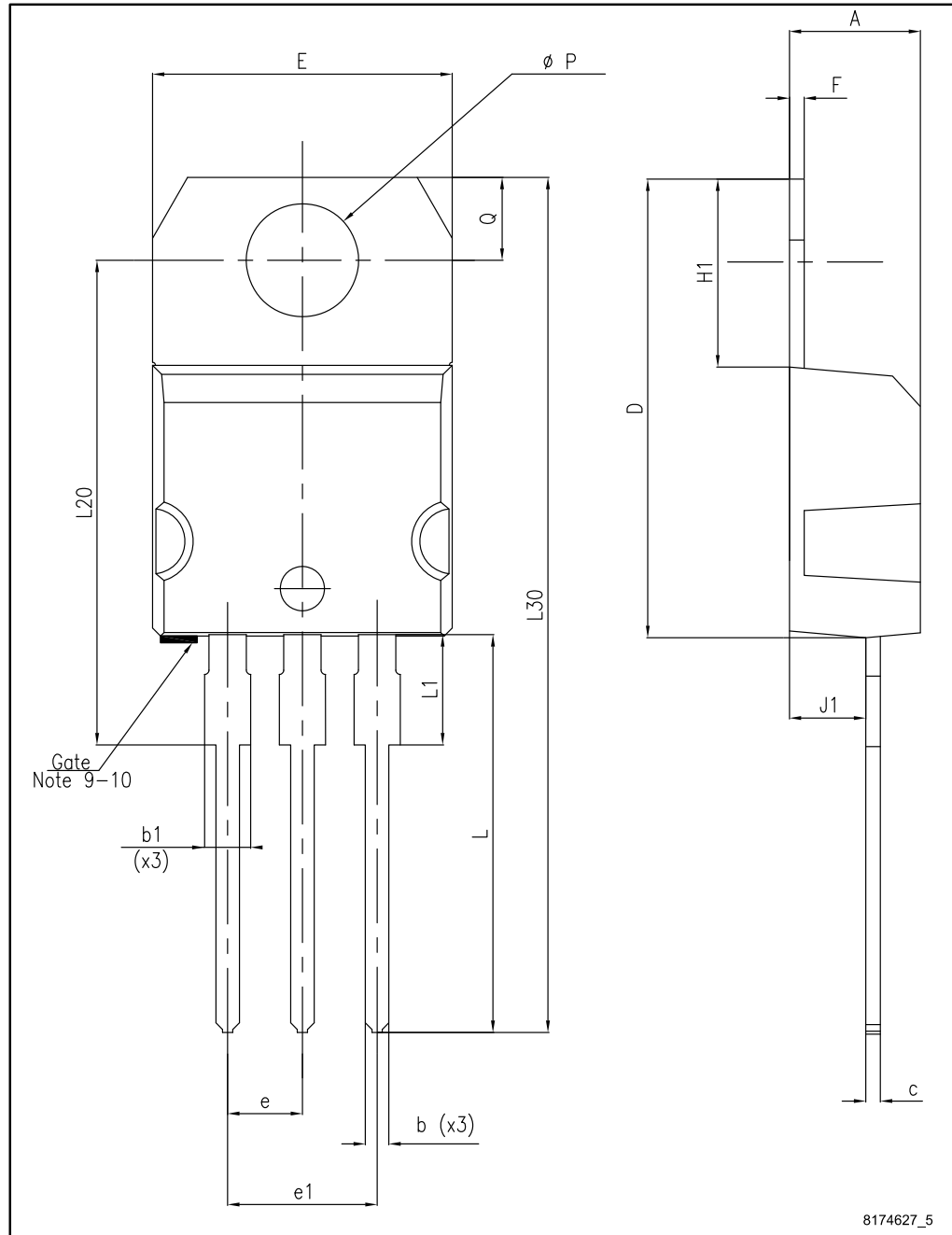
Figure 29: TO-220 (single gauge) package outline
