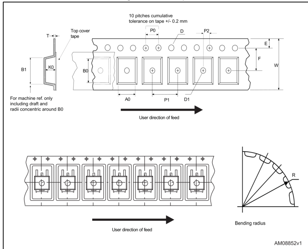
Figure 36: DPAK tape
