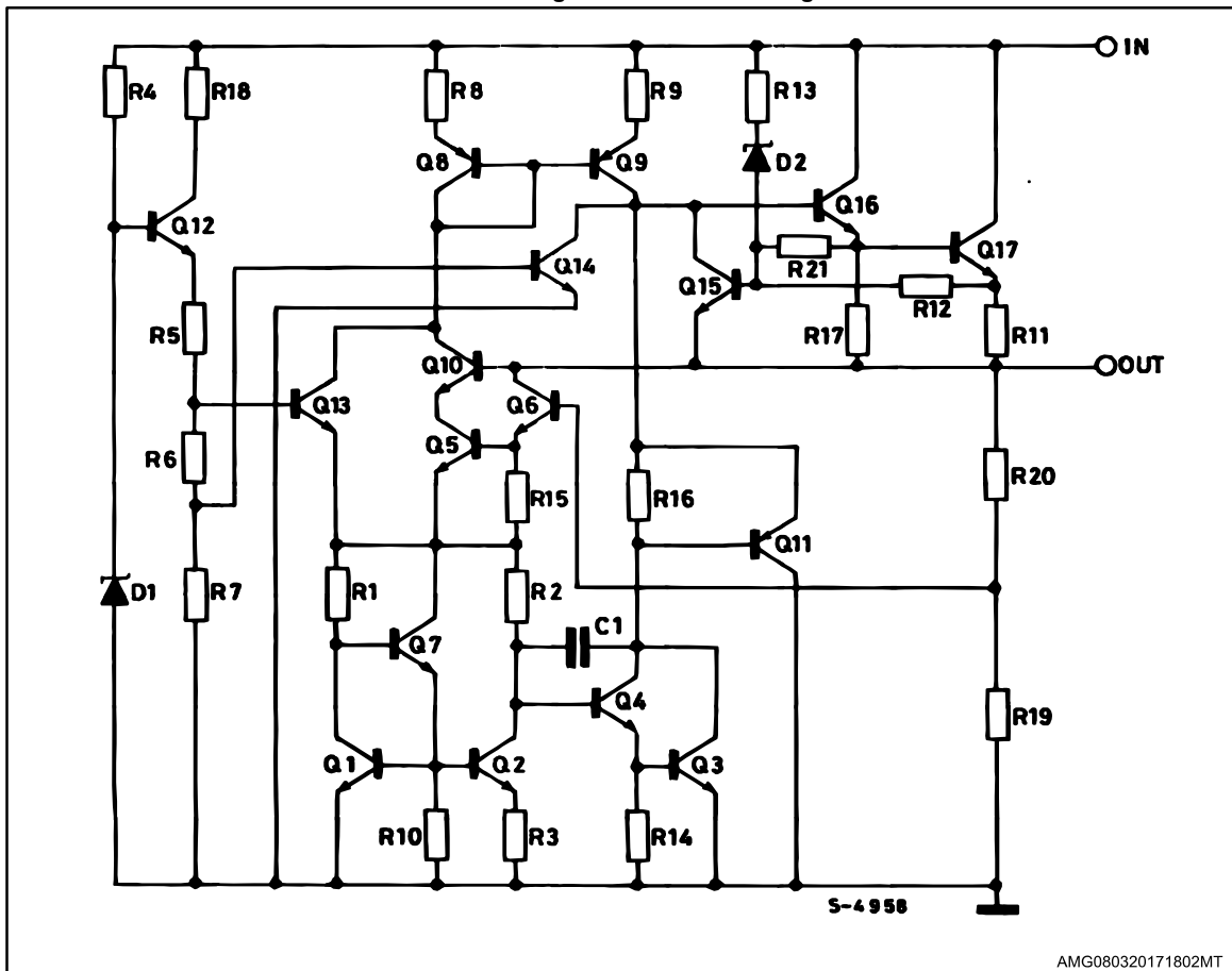
Figure 3: Schematic diagram
