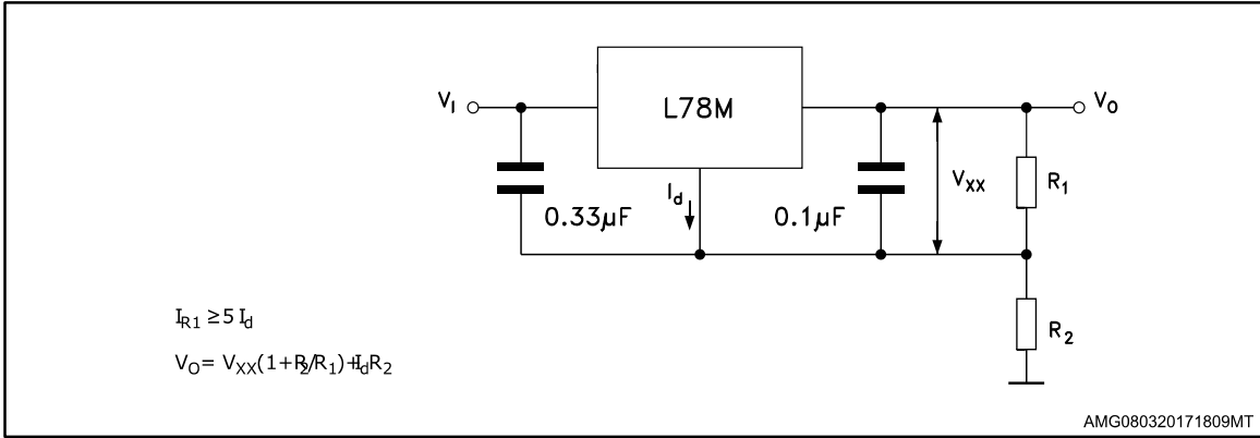
Figure 20: Adjustable output regulator (7 to 30 V)
