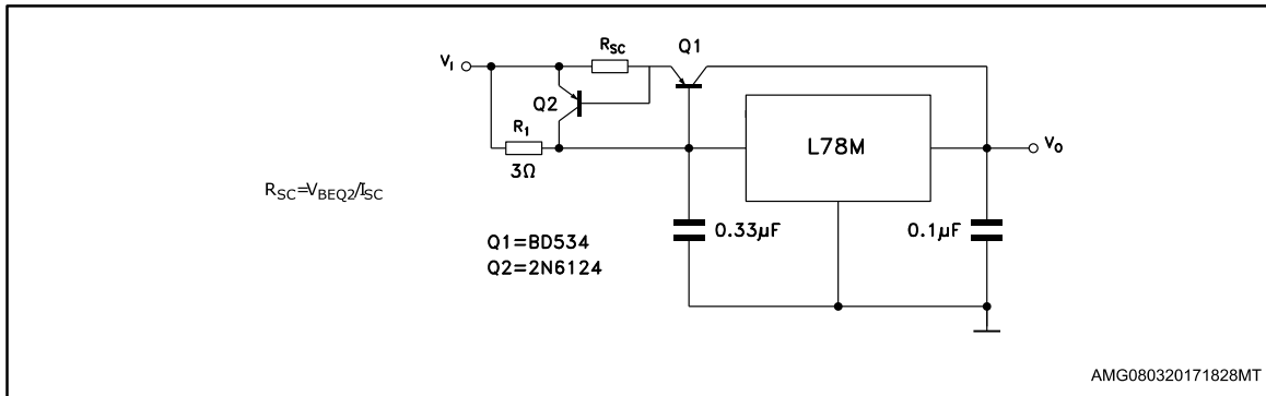
Figure 24: Tracking voltage regulator
