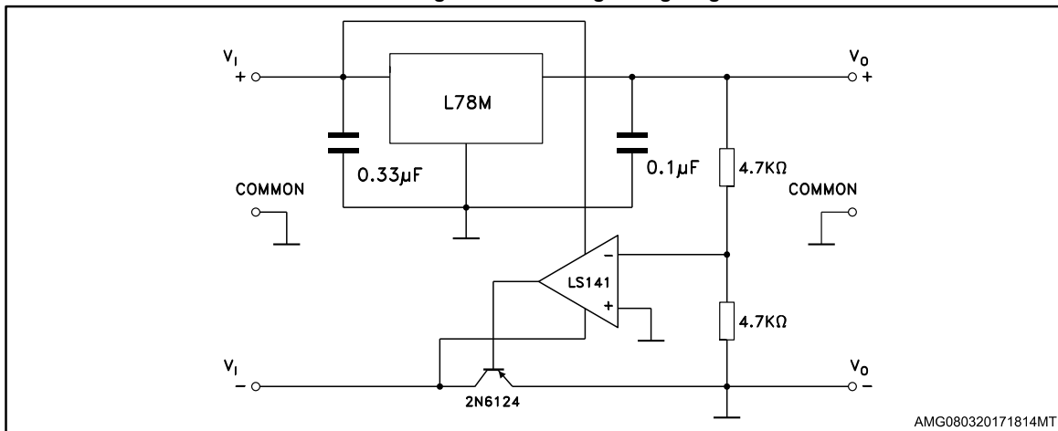
Figure 25: High input voltage circuit
