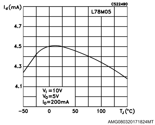
Figure 13: Quiescent current vs junction temperature
