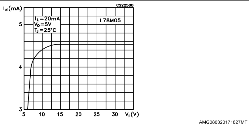
Figure 16: Quiescent current vs input voltage
