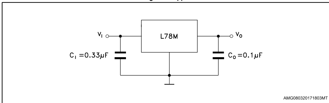
Figure 4: Application circuit
