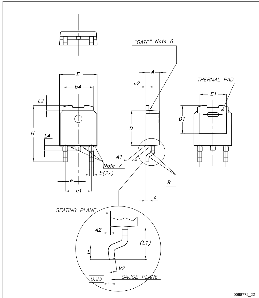
Figure 32: DPAK (TO-252) type A package outline
