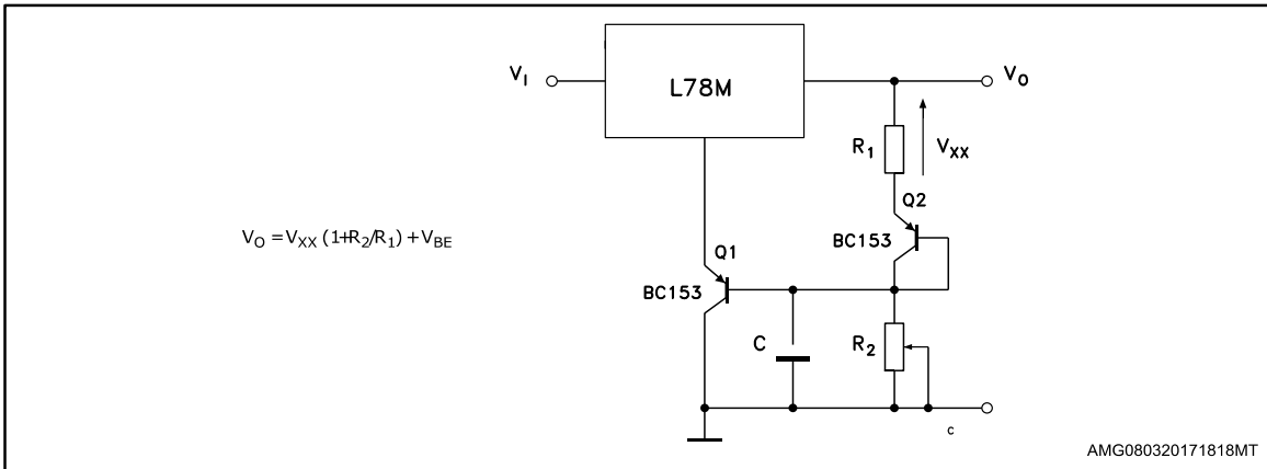
Figure 28: Adjustable output voltage with temperature compensation
