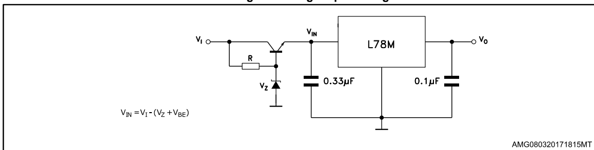
Figure 25: High input voltage circuit
