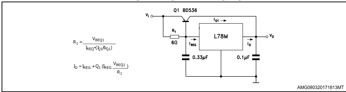
Figure 23: High output current with short circuit protection
